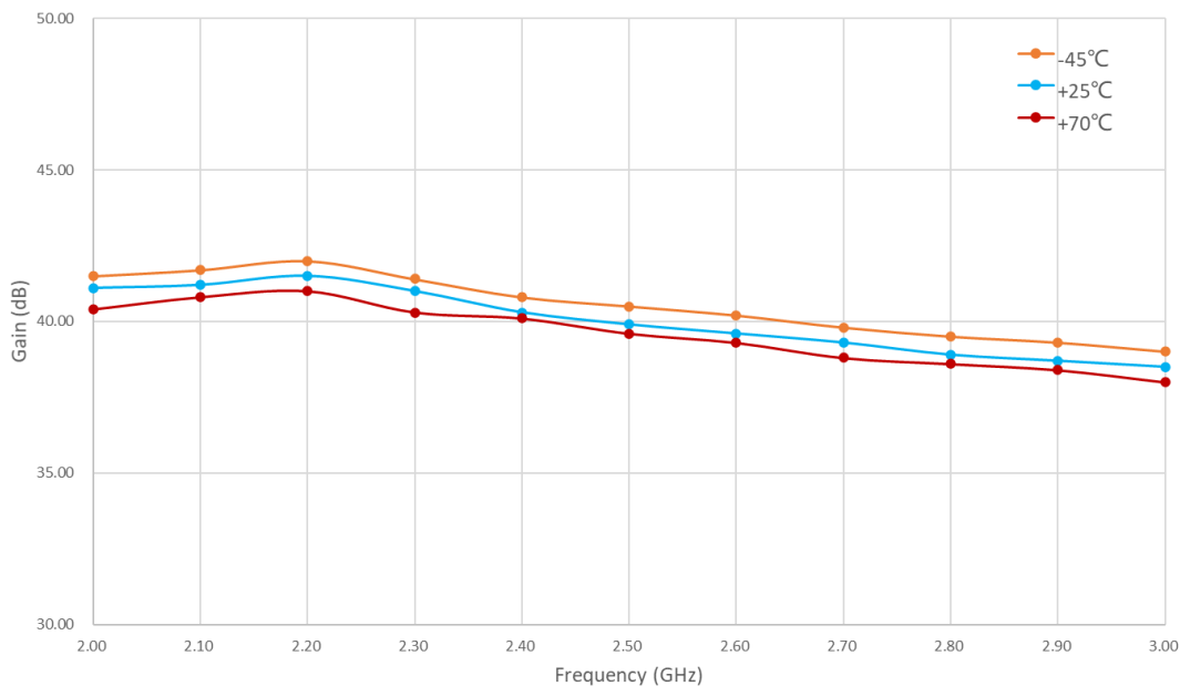
Figure 2: PPA-0200-0300-50 Small Signal Gain Vs Temperature
