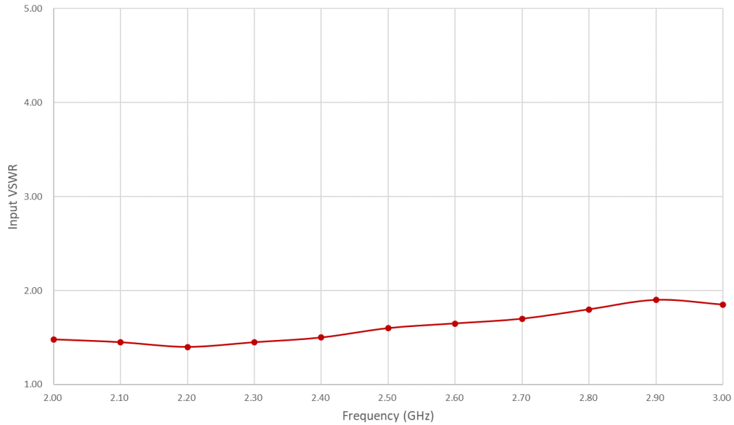
Figure 3: PPA-0200-0300-50 Input VSWR
