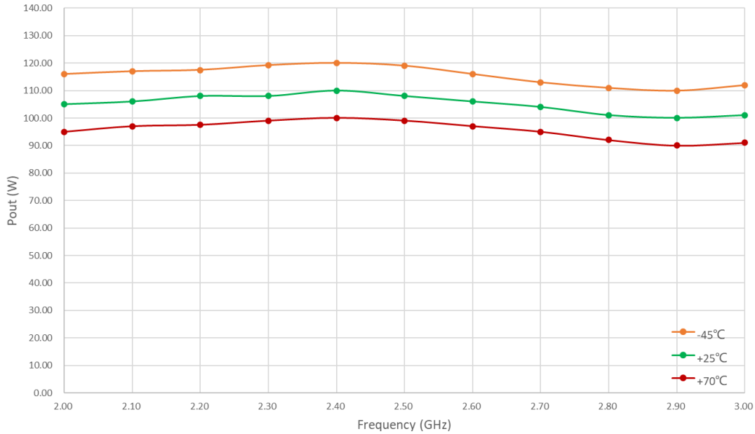
Figure 1: PPA-0200-0300-50 Psat
