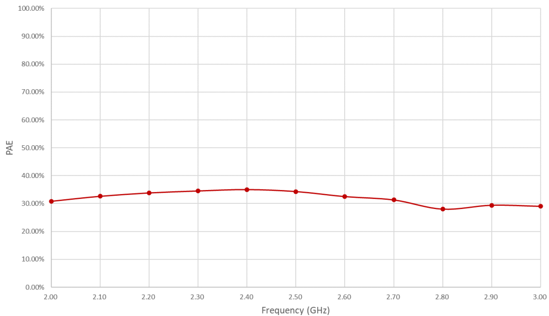
Figure 4: PPA-0200-0300-50 P.A.E
