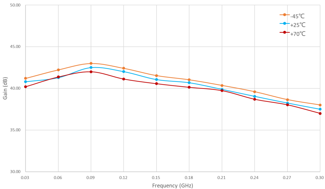
Figure 2: PPA-0003-0030-50 Small Signal Gain Vs Temperature
