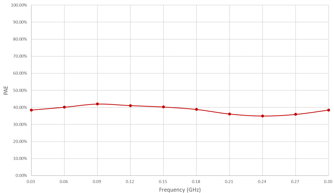
Figure 4: PPA-0003-0030-50 P.A.E
