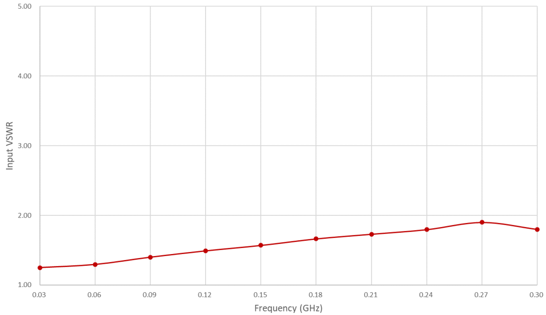
Figure 3: PPA-0003-0030-50 Input VSWR
