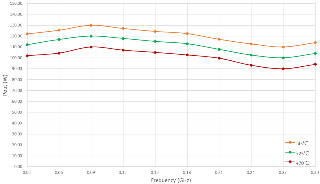
Figure 1: PPA-0003-0030-50 Psat
