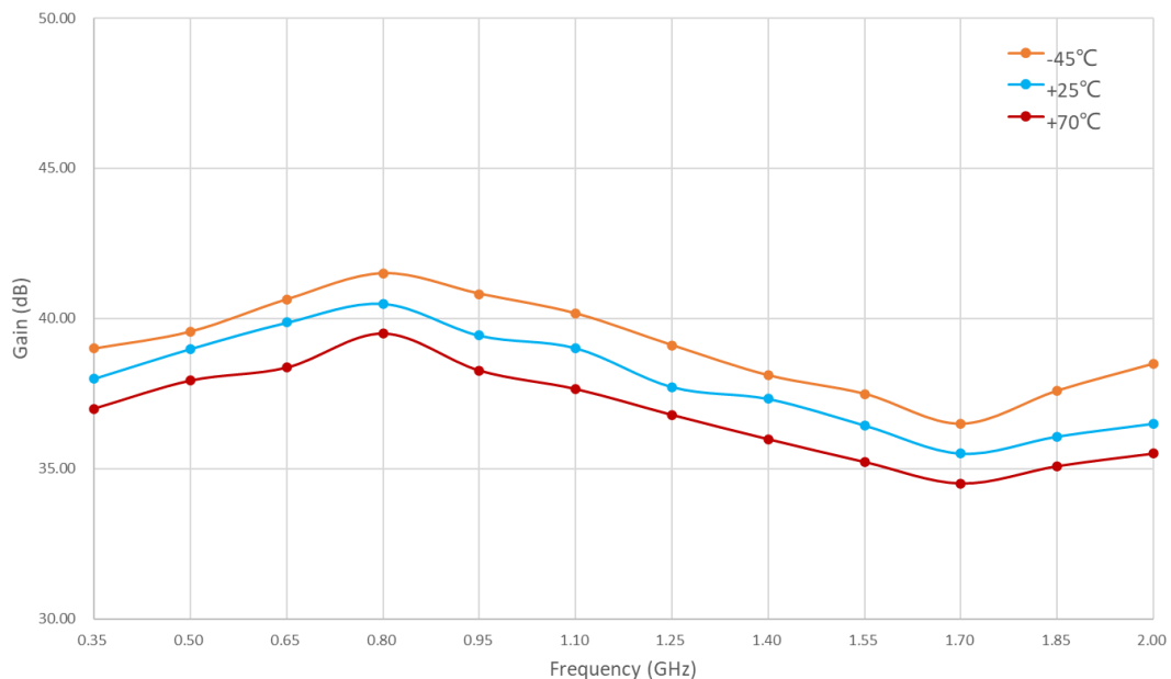
Figure 2: PPA-0035-0200-47 Small Signal Gain Vs Temperature
