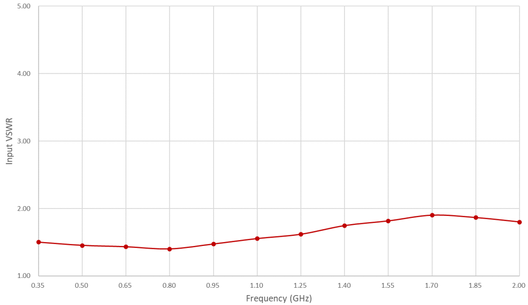
Figure 3: PPA-0035-0200-47 Input VSWR
