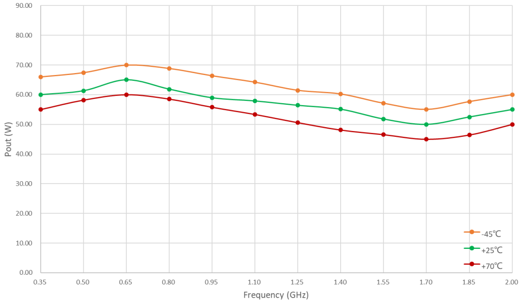
Figure 1: PPA-0035-0200-47 Psat
