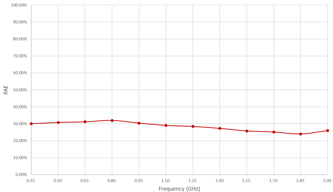
Figure 4: PPA-0035-0200-47 P.A.E
