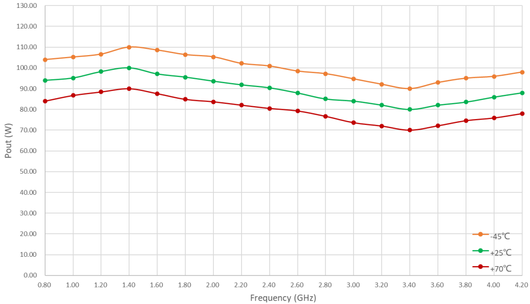
Figure 1: PPA-0080-0420-49 Psat
