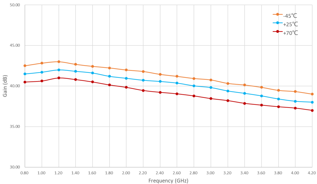
Figure 2: PPA-0080-0420-49 Small Signal Gain Vs Temperature
