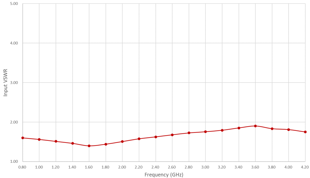
Figure 3: PPA-0080-0420-49 Input VSWR
