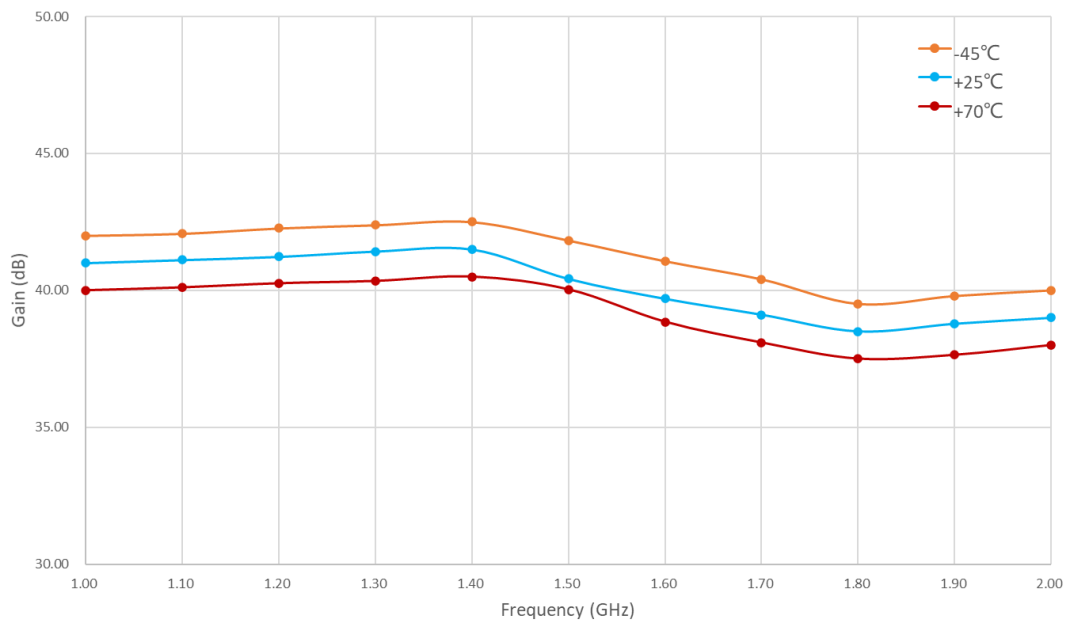
Figure 2: PPA-0100-0200-50-1 Small Signal Gain Vs Temperature
