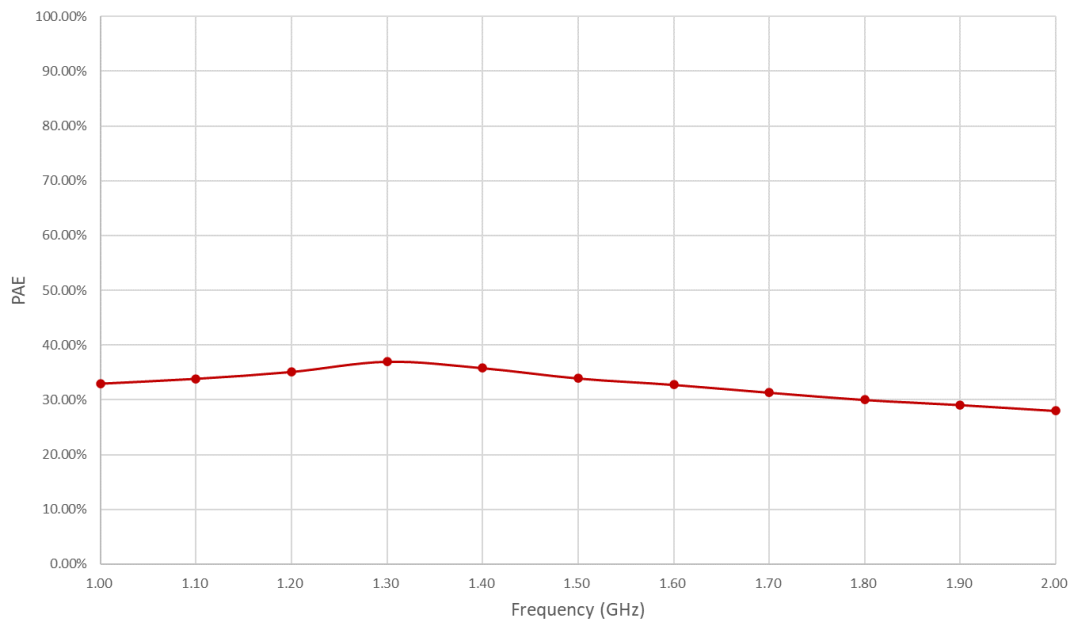
Figure 4: PPA-0100-0200-50-1 P.A.E
