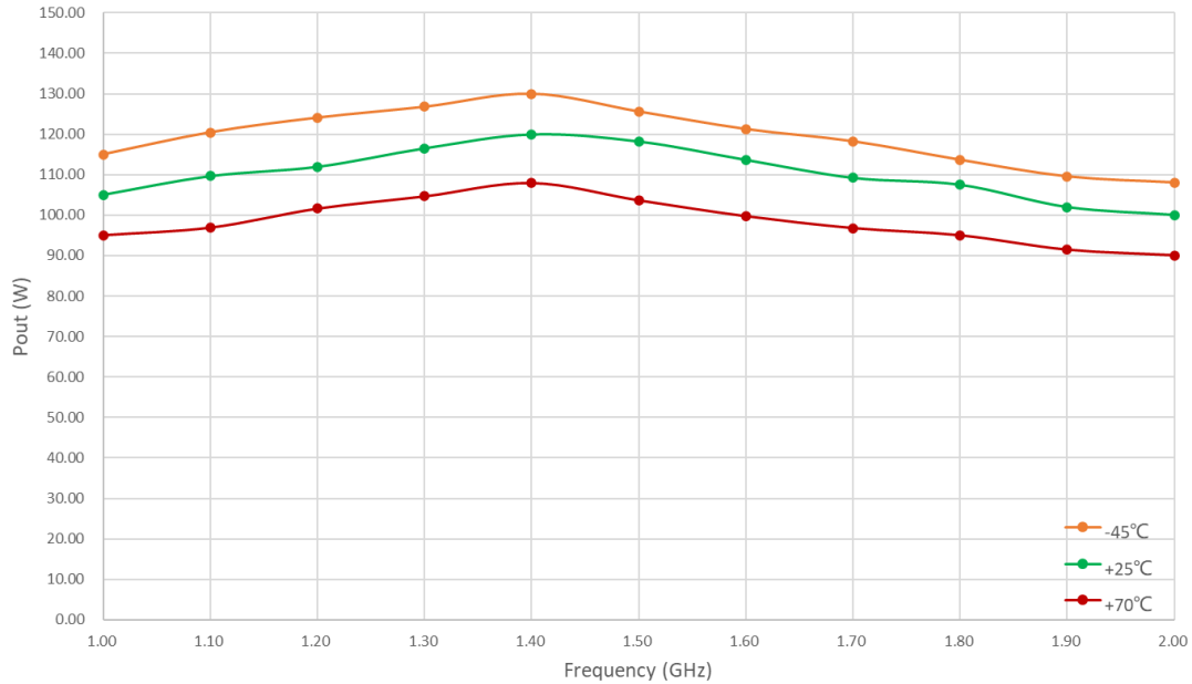
Figure 1: PPA-0100-0200-50-1 Psat
