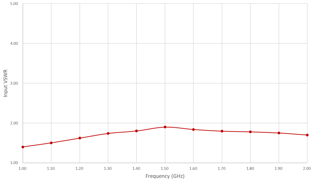
Figure 3: PPA-0100-0200-50-1 Input VSWR
