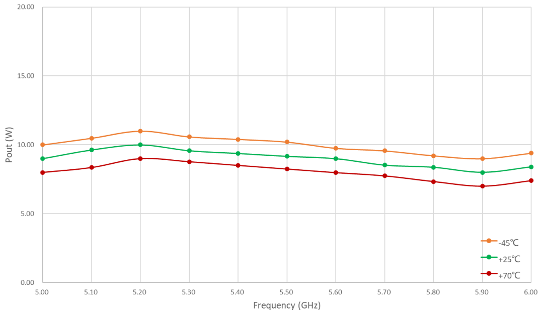
Figure 1: PPA-0500-0600-39 Psat
