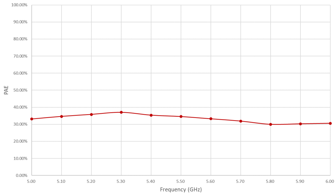
Figure 4: PPA-0500-0600-39 P.A.E
