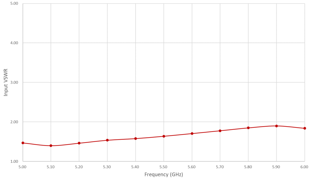
Figure 3: PPA-0500-0600-39 Input VSWR
