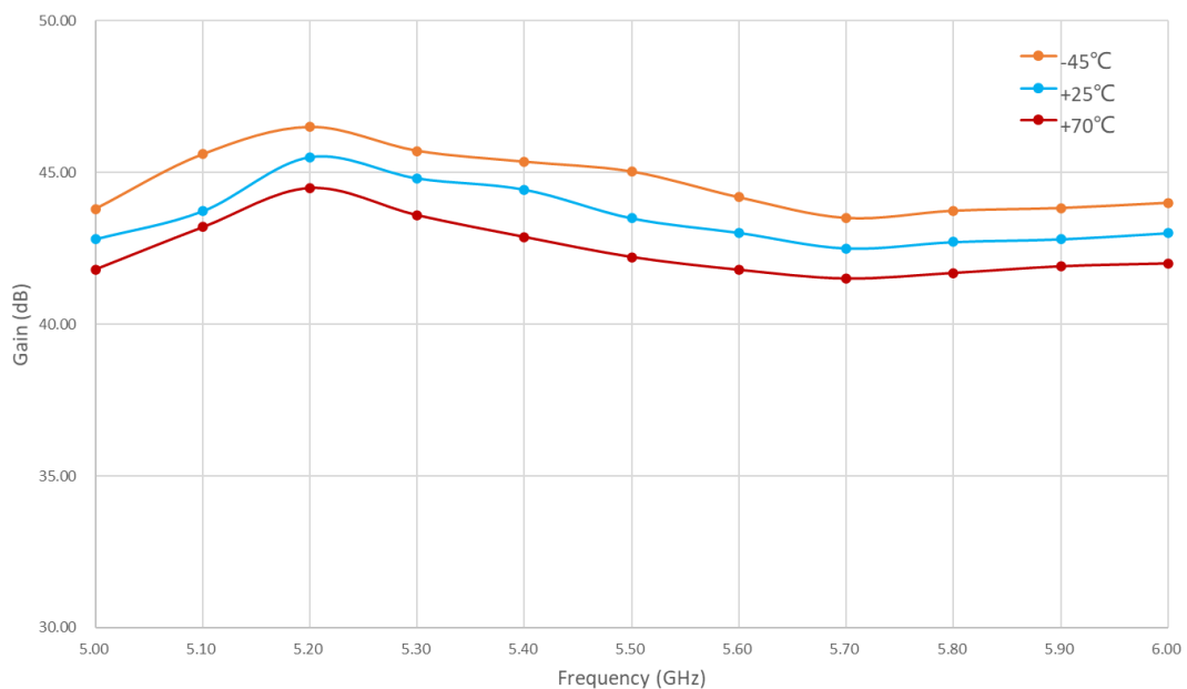
Figure 2: PPA-0500-0600-39 Small Signal Gain Vs Temperature
