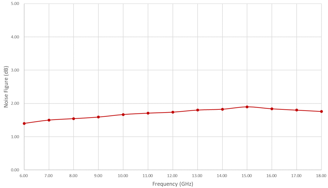
Figure 1: PLNA-0600-1800-15 Noise Figure
