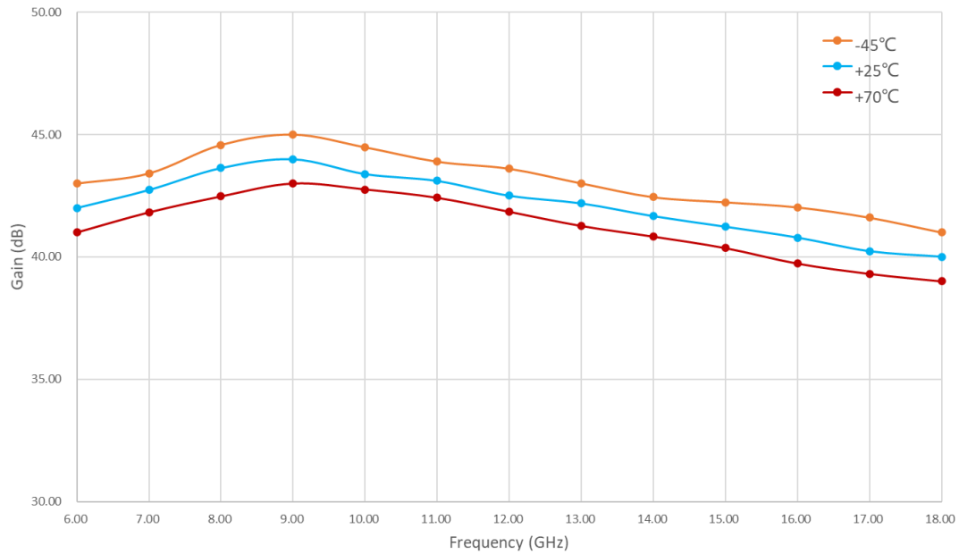
Figure 3: PLNA-0600-1800-15 Small Signal Gain Vs Temperature
