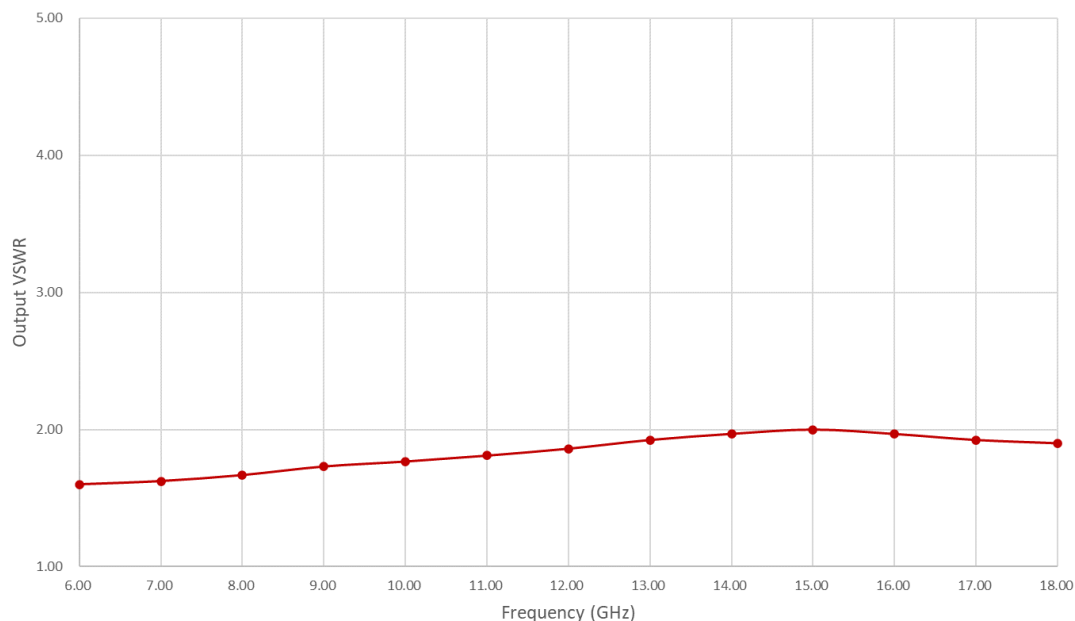
Figure 5: PLNA-0600-1800-15 Output VSWR
