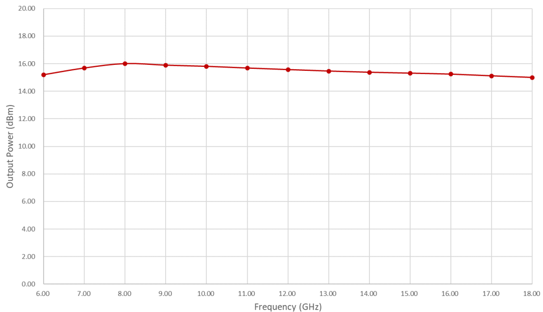
Figure 2: PLNA-0600-1800-15 P1dB
