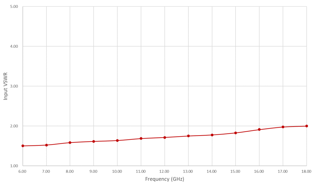
Figure 4: PLNA-0600-1800-15 Input VSWR
